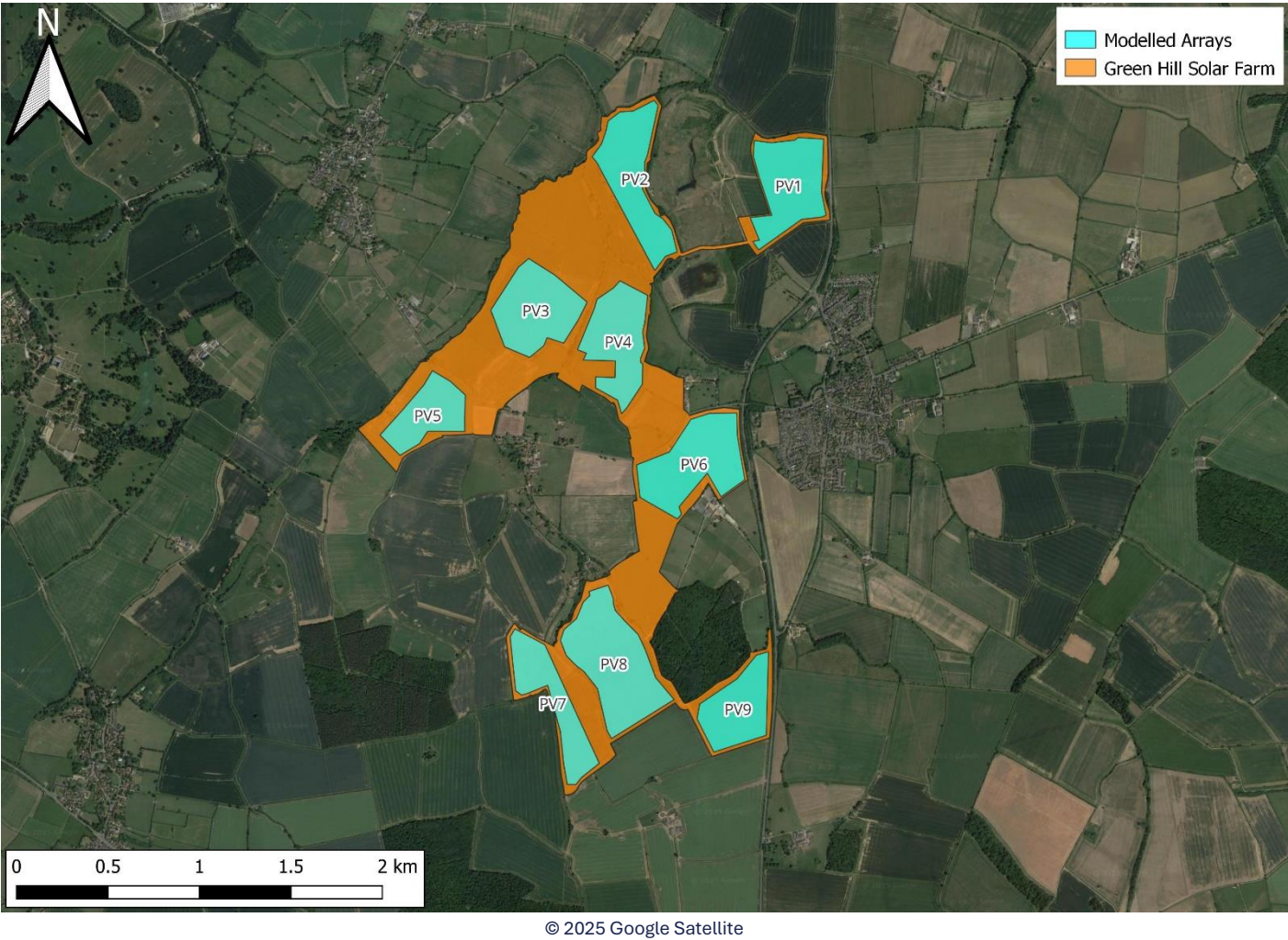
Figure 2.3: Modelled PV Panels at Green Hill F
